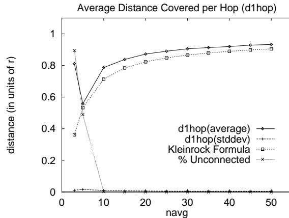
Fig. 2. Theoretical and experimental values for the average distance covered in one communication hop d_{hop} , for different expected local neighborhoods n_{local} . There is significant improvement below n_{local} = 15 , after which increasing the neighborhood size has diminishing returns.
